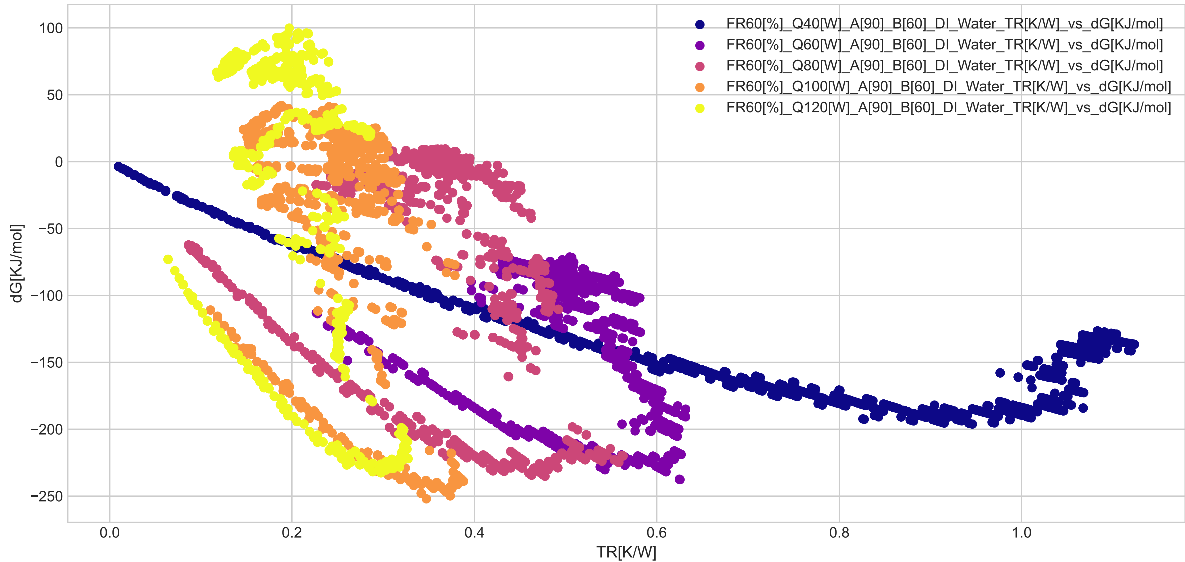
FR [60]% - Q [ 40 60 80 100 120]W - alpha [90] - beta [60] - DI_Water
